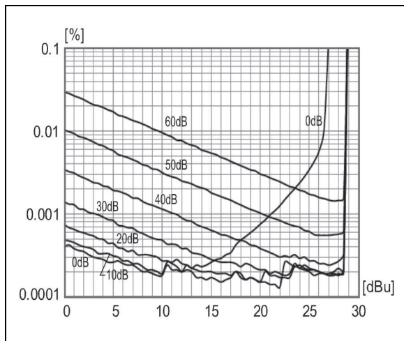
Figure 6. THD + Noise vs Level f = 1 \text{ kHz} , BW: 22 Hz to 22 kHz
