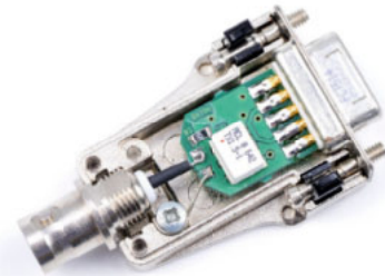
PCB in a metal hood PCB in Vollmetallhaube
