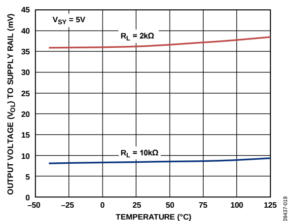
Figure 24. Output Voltage ( V_{OL} ) to Supply Rail vs. Temperature
