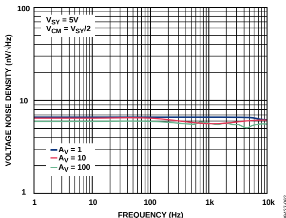
Figure 66. Voltage Noise Density vs. Frequency with Different Gain Configurations
