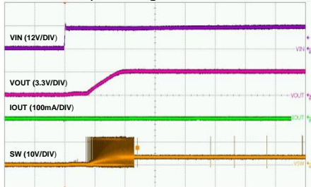
Time-500μs/div
