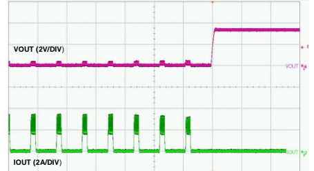
Time-5ms/div
