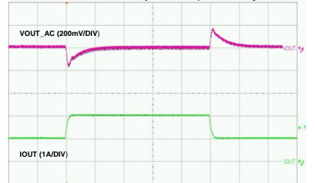
Time-100μs/div
