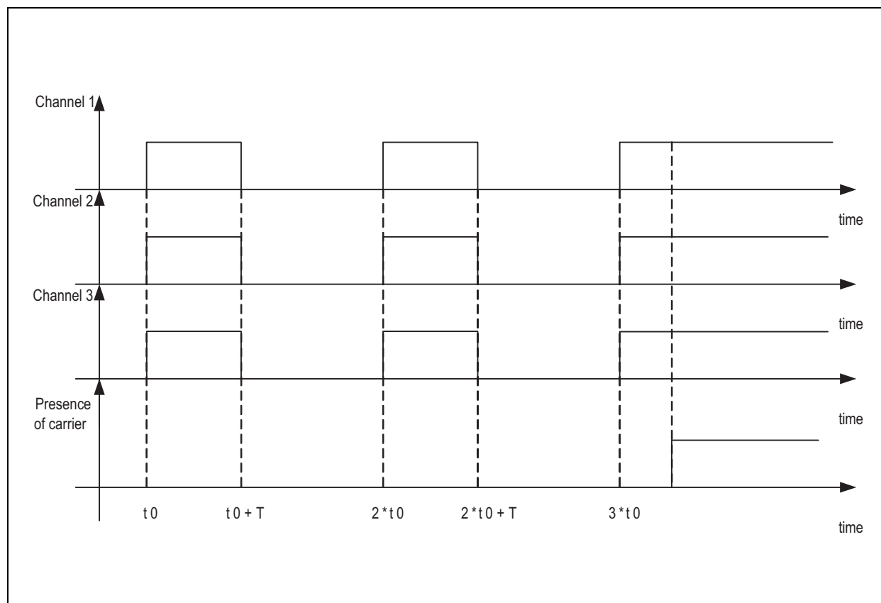
Figure 18: ON/OFF Mode
