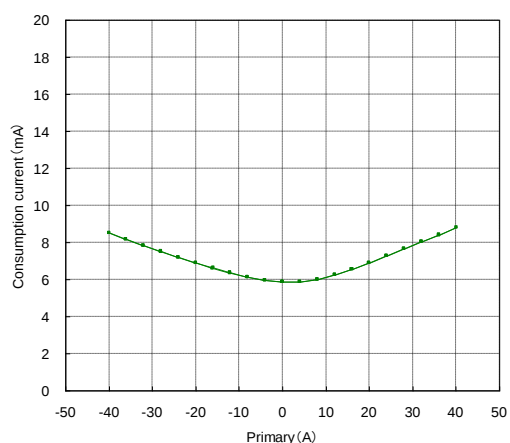
Fig.9-3 Consumption Current
