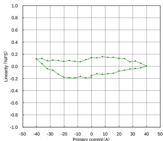
Fig.9-2 Linearity
