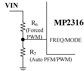
Figure 3—Mode Selection
