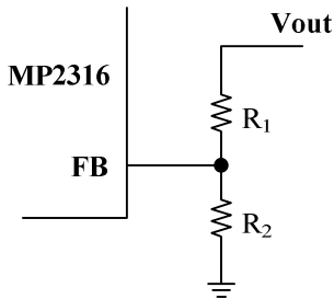
Figure 9—Feedback Network
