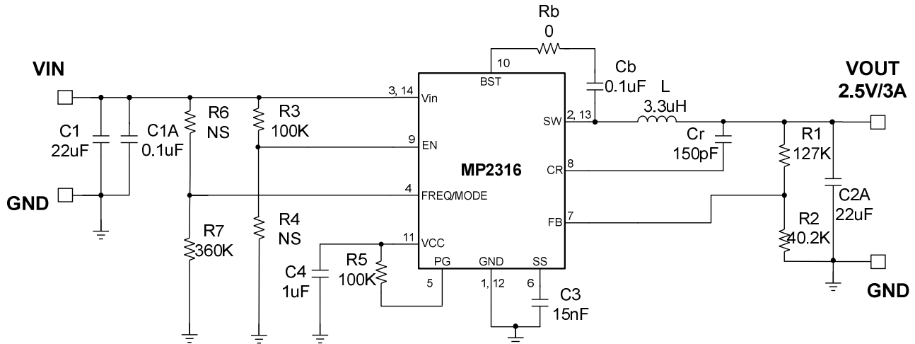
Figure 18— V_{IN}=12V , V_{OUT}=2.5V , I_{OUT}=3A , F_S=500kHz
