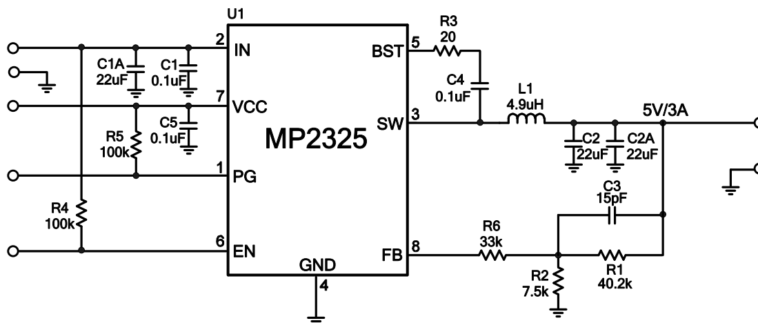
Figure 8: V_o=5V , I_o=3A
