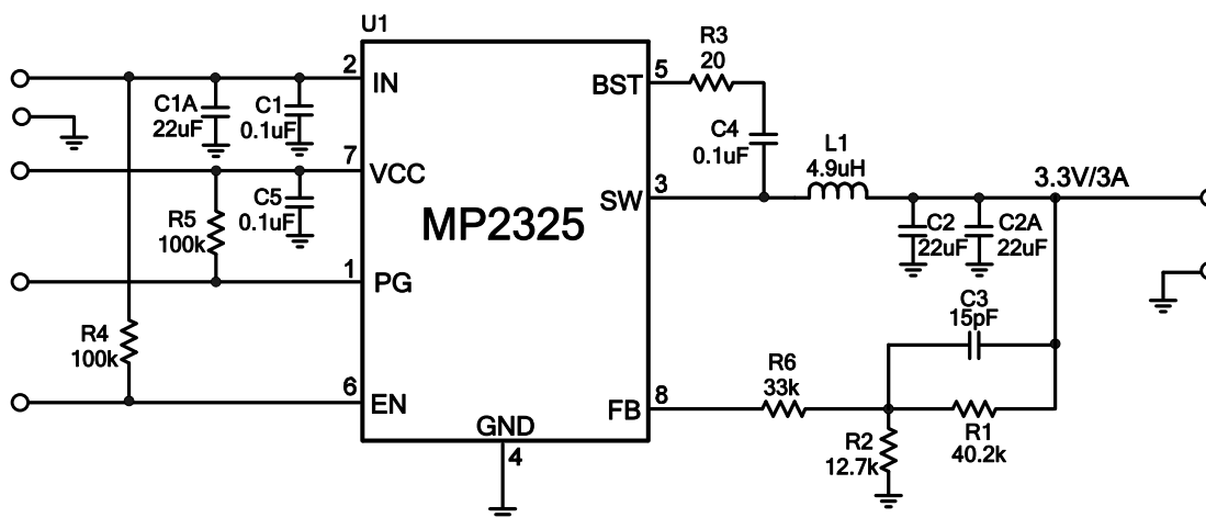
Figure 9: V_o=3.3V , I_o=3A
