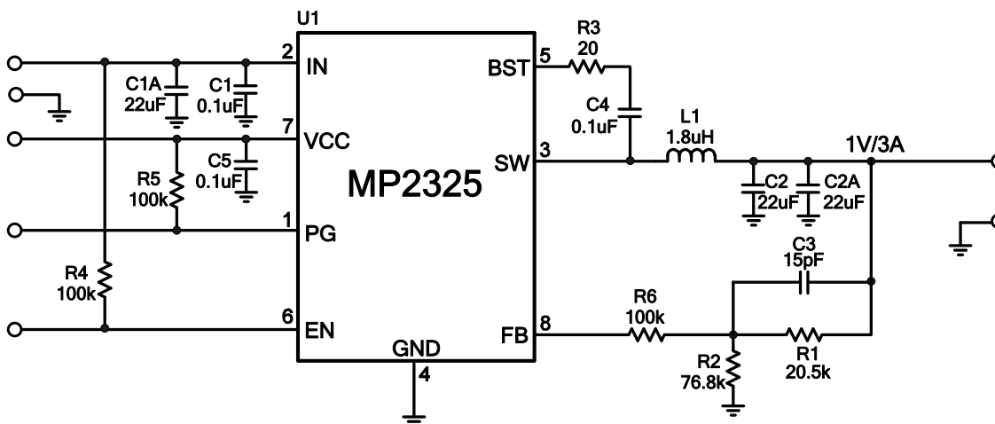
Figure 13: V_o=1V , I_o=3A
