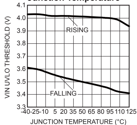
V IN UVLO Threshold vs. Junction Temperature
