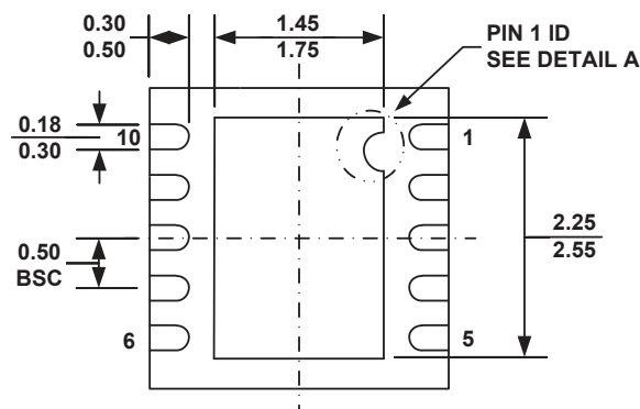
QFN-10 (3mmx3mm)
