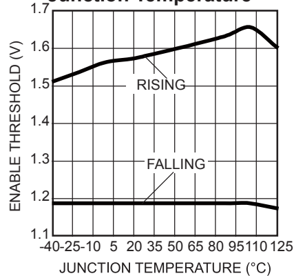
Enable Threshold vs. Junction Temperature
