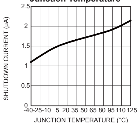
Shutdown Current vs. Junction Temperature
