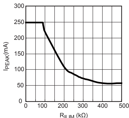
I PEAK vs. R LIM
