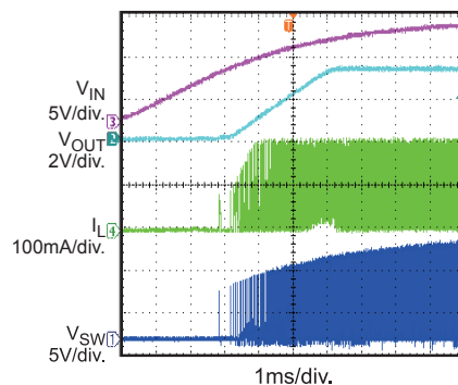
Startup Through Input Voltage I_{OUT} = 100mA
