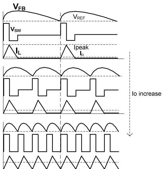
Figure 2 – PWM Control
