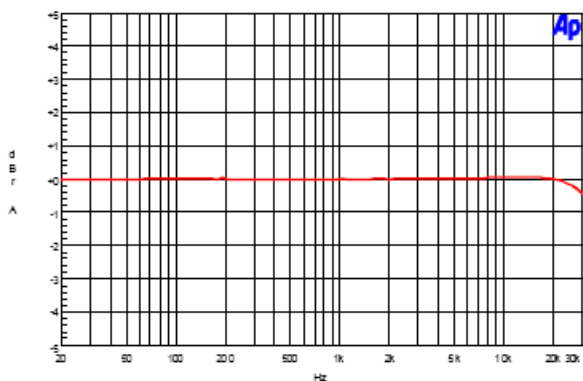
15. Frequency Response ( V_o = 1.0\text{V}_{\text{rms}} )
