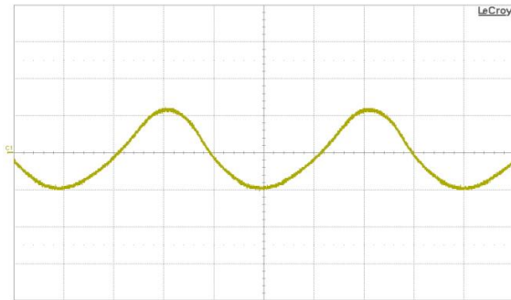
Fig. 15: Input reflected ripple current, i_c (1 A/div.), measured at input terminals at full rated load current and V_{in} = 48 V. Refer to Fig. 14 for test setup. Time scale: 1 \mu s/div.
