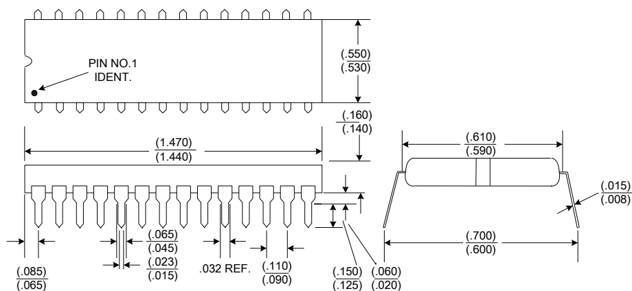
Figure 26 - 28 Pin Plastic Dip Package Dimensions
