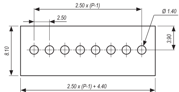
PCB Layout
