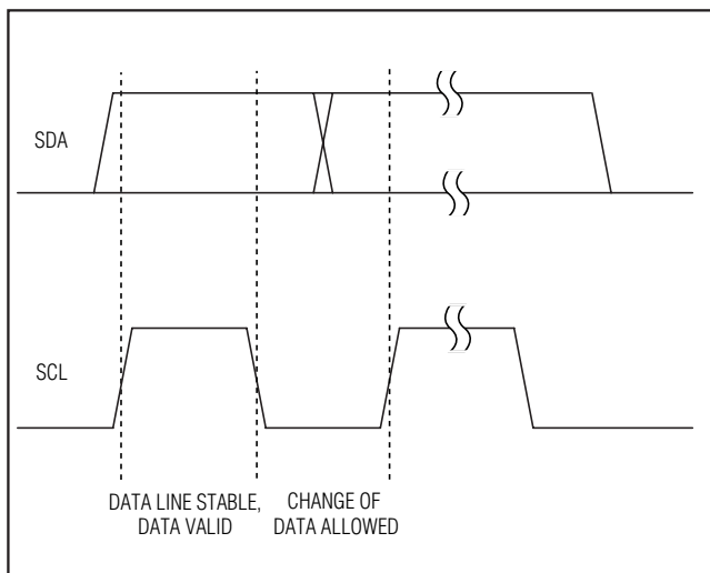
Figure 6. Bit Transfer
