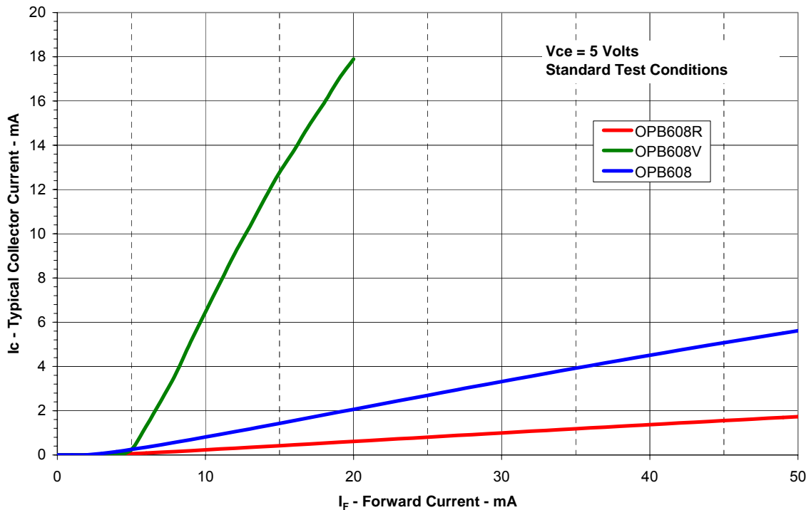
Collector Current vs Diode Forward Current
