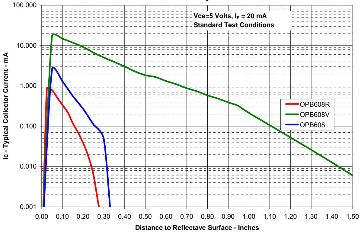
Collector Current vs Object Distance
